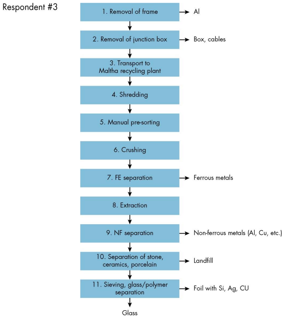
Fig. 3.1 Process flow diagram of the Maltha glass recycling plant in Belgium (Wambach et al. 2018). c-Si PV modules are treated mechanically in several process steps in order to recover the aluminium frame, the junction box, cables, ferrous and non-ferrous metals as well as glass.
