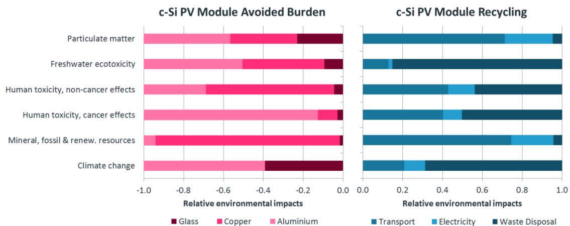
Fig. 4.1 Relative contributions of recovered materials to the potential benefits ( left ) and relative contributions of the recycling processes to the environmental burdens ( right ) of first generation c-Si PV module recycling based on data from four European recyclers.
